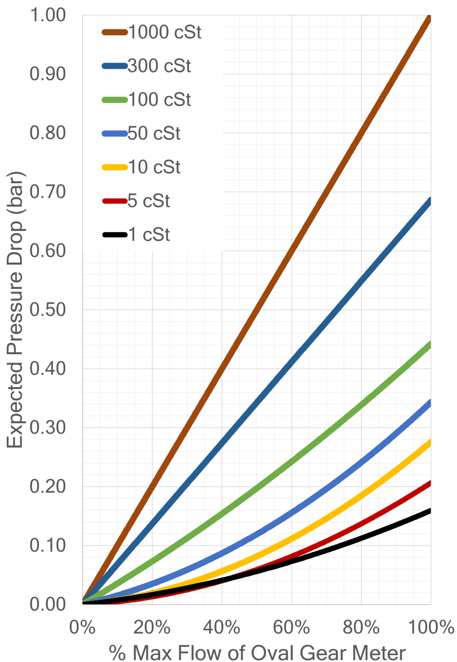
Titan Enterprises Oval Gear Pressure Drop Information
